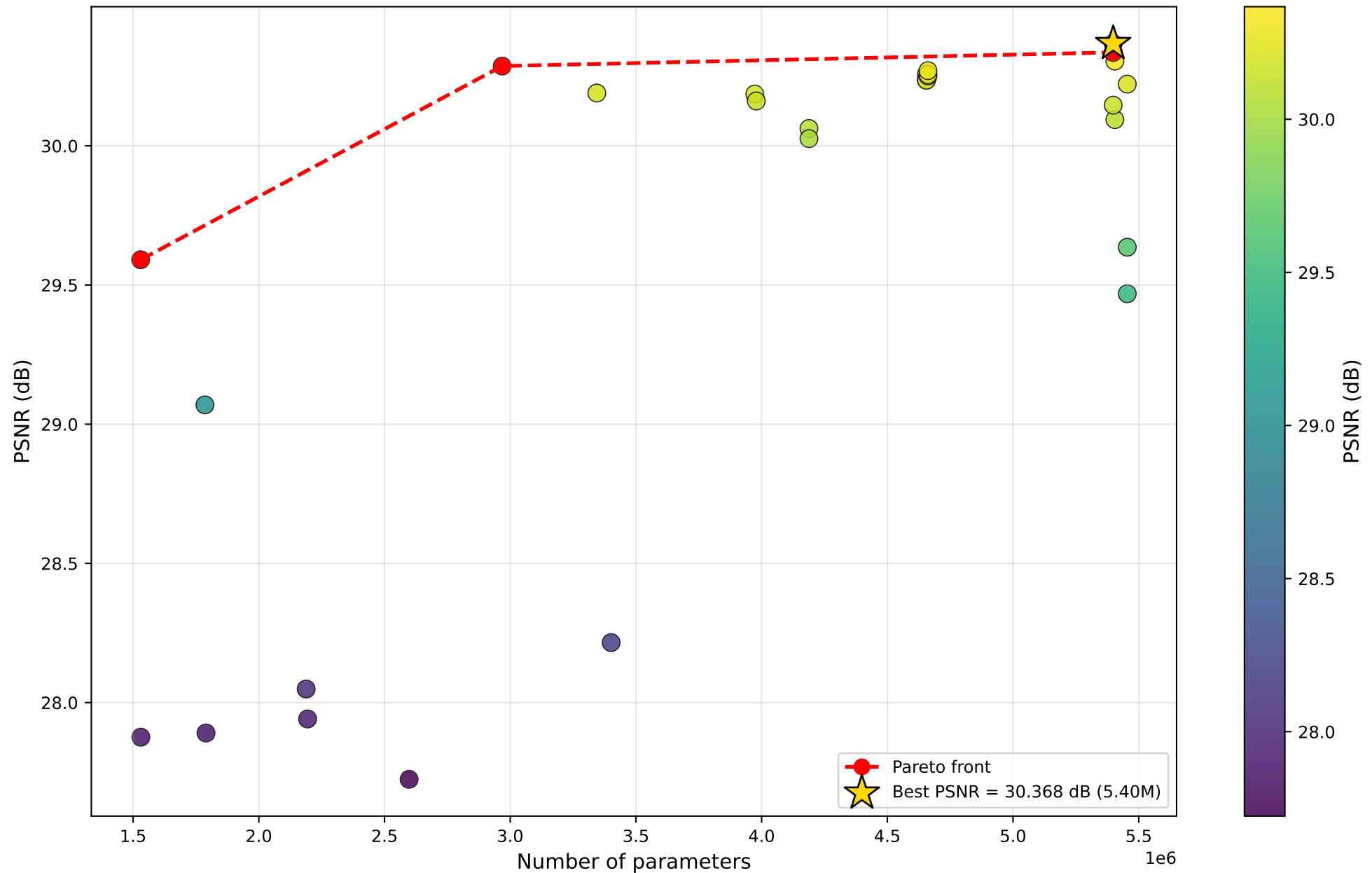
PSNR vs #Parameters — WaveletAttention
